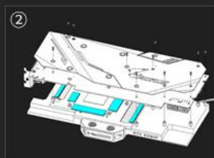
the GPU backplane hole fit to the water block base hole, then lock by screws
